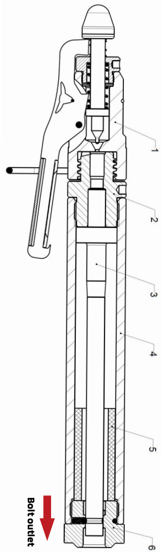
fig.: captive bolt stunner Bullen Blitz (unloaded and untensioned)
